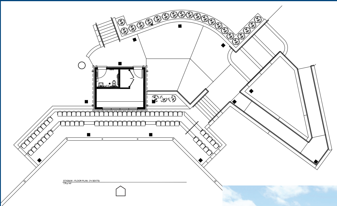
New Press Box and Seating
