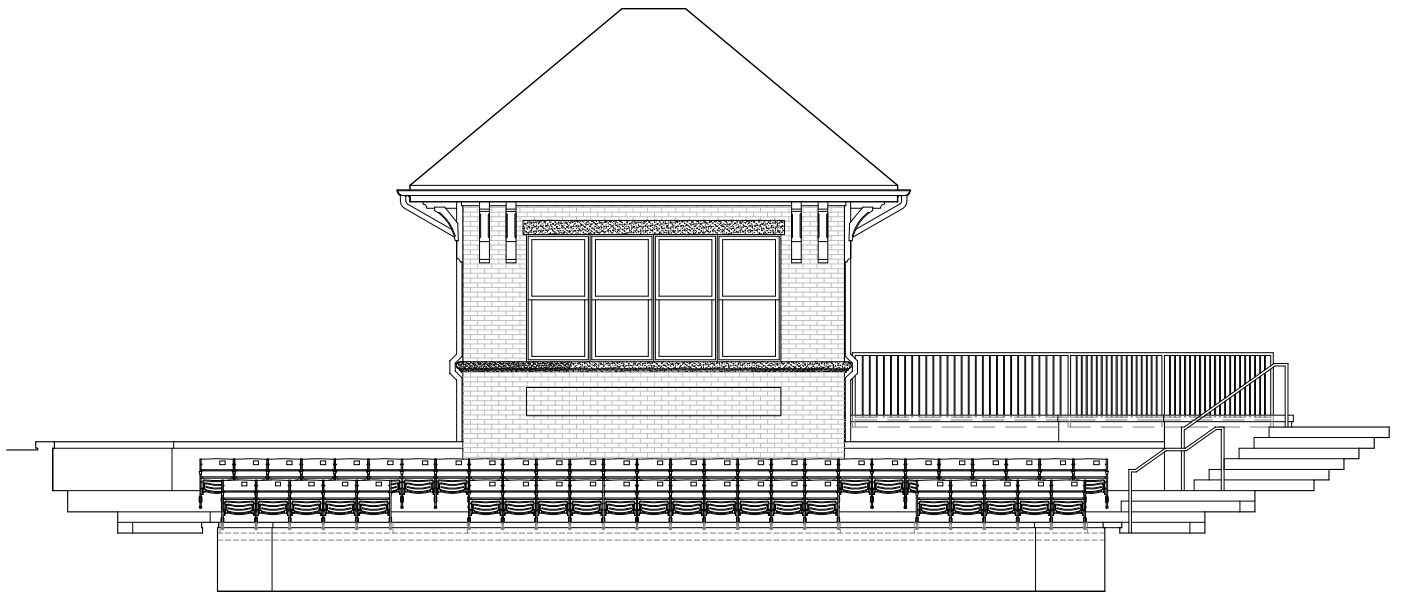
3 STADIUM CENTER BLEACHER ELEVATION (FIELD SIDE) 1/4" = 1'-0"
